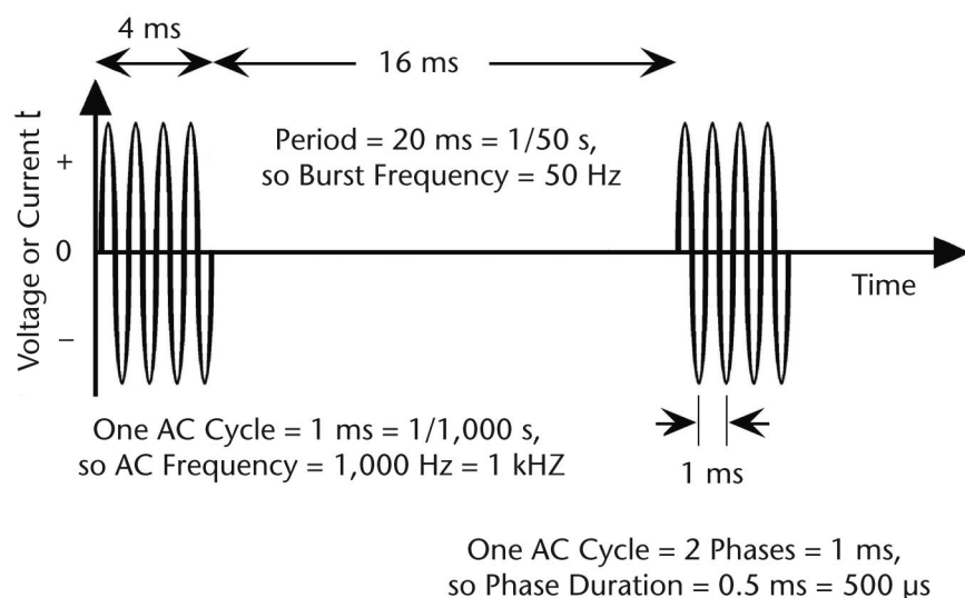
Figure 2. An example of burst-modulated alternating current. A minimum of 5 parameters must be specified in order to describe the waveform. In this example, the waves are sinusoidal, the alternating current (AC) frequency is 1 kHz, the bursts are rectangular, the burst frequency is 50 Hz, and the burst duration is 4 milliseconds.
