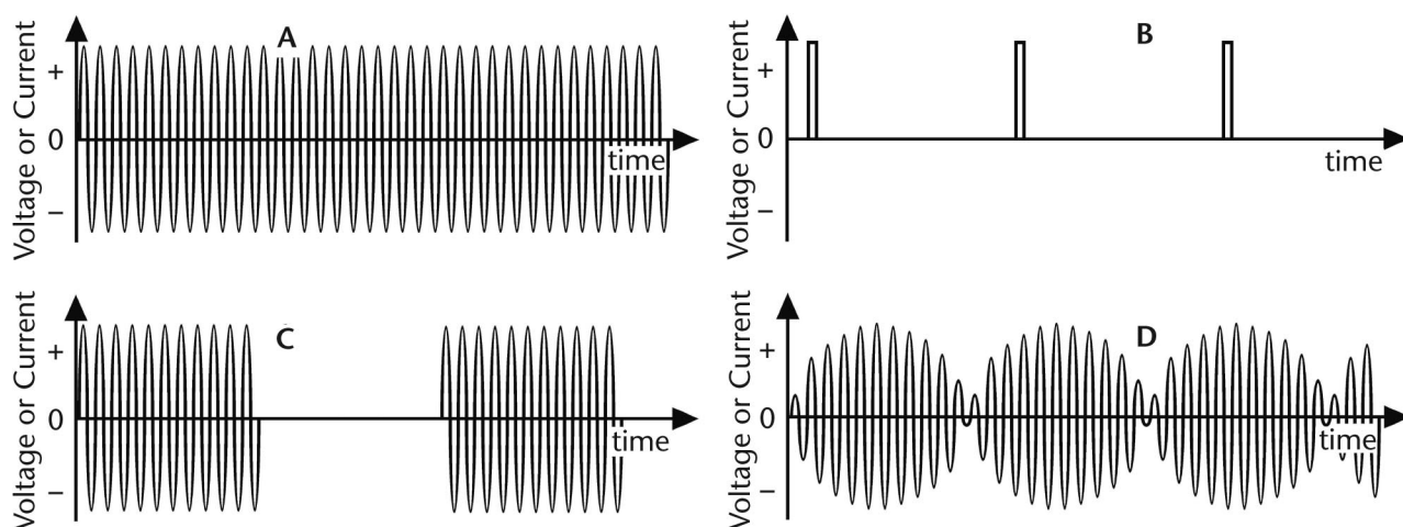
Figure 1. (A) Steady, unmodulated alternating current; (B) monophasic pulsed current; (C) burst-modulated alternating current with rectangular burst modulation; and (D) burst-modulated alternating current with sinusoidal modulation.
