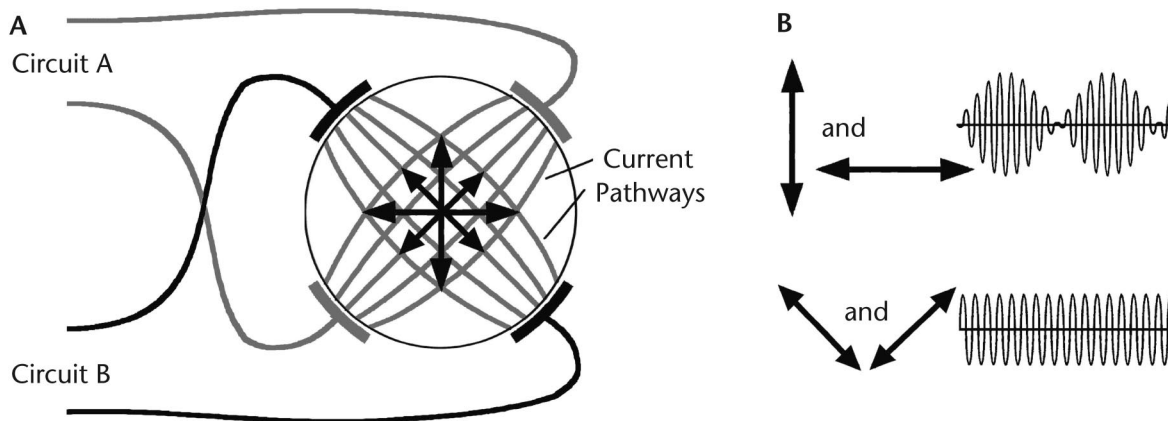
Figure 3. (A) Interferential currents are claimed to produce maximum stimulation in the region of intersection of the 2 diagonally opposed currents, as shown. (B) The actual stimulation intensity experienced by nerve fibers has maximum modulation if the fibers are oriented optimally and zero modulation when fibers are oriented along one of the current pathways.
